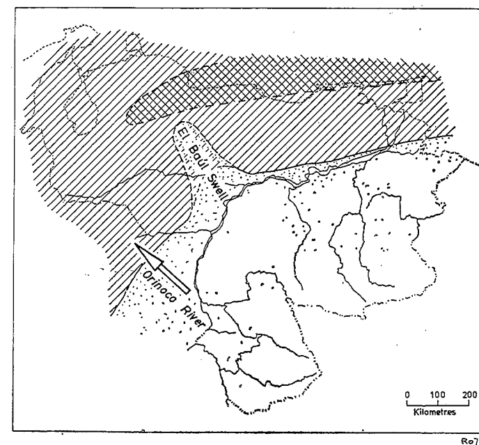
Fig. 1. Late Cretaceous time. See MENCHER et al. (1953: 698, Figure 3) and PATTERSON and WILSON (1953: 2711).
