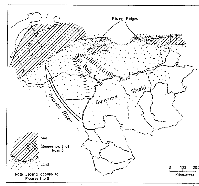
Fig. 2. Early Eocene time. See MENCHER et al. (1953: 704, Figure 4).
