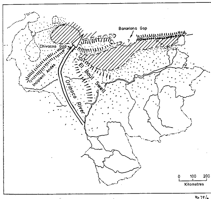
Fig. 4. Early Oligocene time. Deposition of La Pascua-Roblecito and of basal Naricual, including Areo shale.
