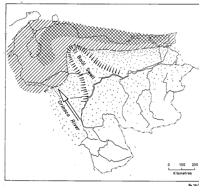
Fig. 3. Late Eocene time. See MENCHER et al. (1953: 709, Figure 5).
