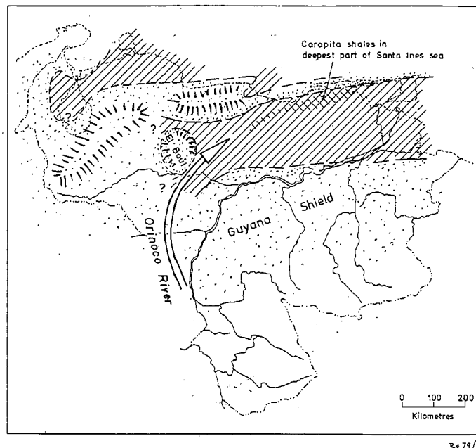
Fig. 5. At close of early Oligocene time and during Oligocene time in general. Beginning of Chaguaramas Oficina deposition.
